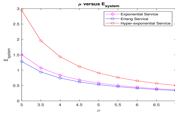
Figure 5: Service rate versus the expected system size for all service distribution with Exponential arrival
