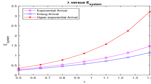
Figure 3: Arrival rate versus the expected system size for all arrivals distribution with Erlang phase service
